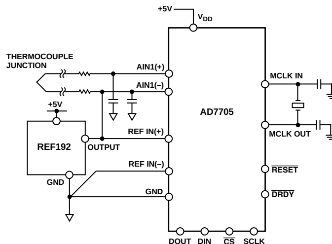
Figure 23. Temperature Measurement Using the AD7705
